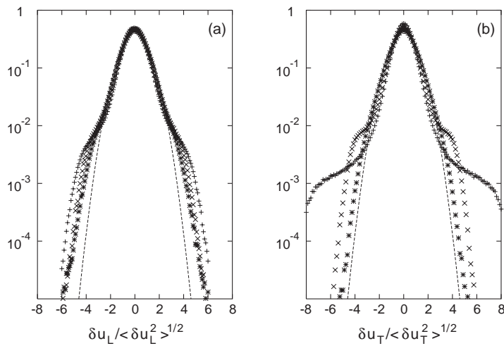
Fig. 4 – Probability density functions of longitudinal (a) and transverse (b) velocity differences at separations \ell = 0.05 (+), \ell = 0.1 (x) and \ell = 0.2 (*) at time t = 10^{-2} . The dashed line represents the Gaussian distribution.
