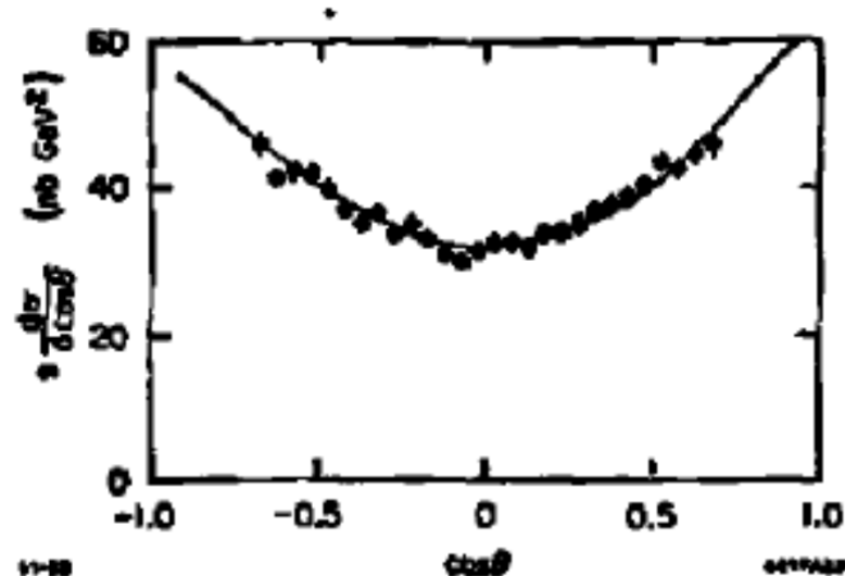
Fig. 15, MARK II e^+e^- \rightarrow u^+u^- at \langle E_{\text{c.m.}} \rangle^4 = 5.847 compared to 1 + \cos^2\theta .
