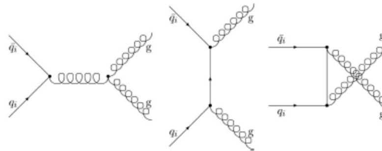
Figure 5: Feynman diagrams for q_i \bar{q}_i \rightarrow gg
