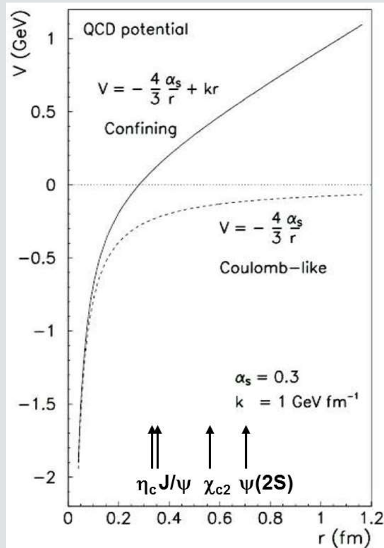
Cornell potential
