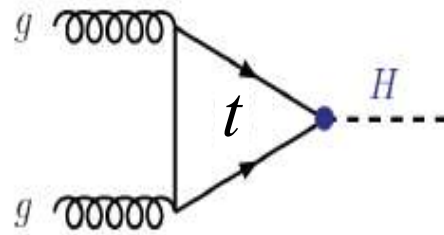
Gluon-Gluon fusion
