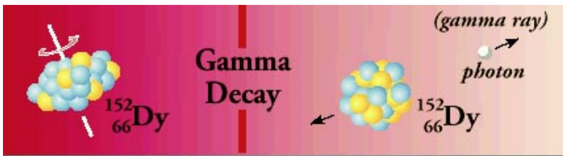
Fig. 3-6. A gamma ( \gamma ) decay.
