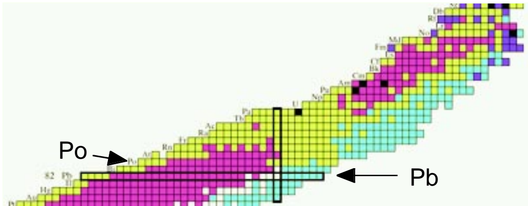
Fig. 3-4. Upper end of the Chart of the Nuclides
