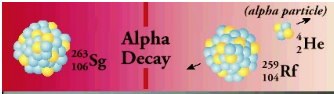
Fig. 3-3. An alpha-particle decay
