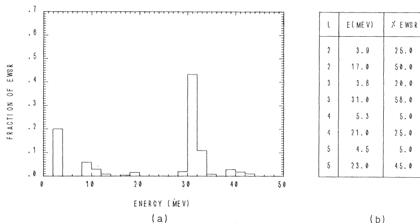
FIG. 1. Oscillator-strength distribution for isoscalar excitations in 40 Ca. In (a) we show the octupole strength distribution in percent of the classical sum rule per 2-MeV interval. It is the result of a random-phase approximation, diagonalizing a separable interaction in a harmonic-oscillator basis including particle-hole excitations up to 50 MeV (cf. Ref. 2). On the basis of this and similar diagrams for other multipolarities the spectrum shown in (b) was constructed. It collects the strength for each multipolarity, L , into a low- and a high-lying collective state with the energies E and transition probability which is given in terms of the percentage of the energy-weighted sum rule (% EWSR). The width assigned to each of the high-lying levels was 4 MeV while the low-lying levels were ascribed a nonlinear damping with s_\lambda = \frac{1}{3} (cf. Ref. 1).
