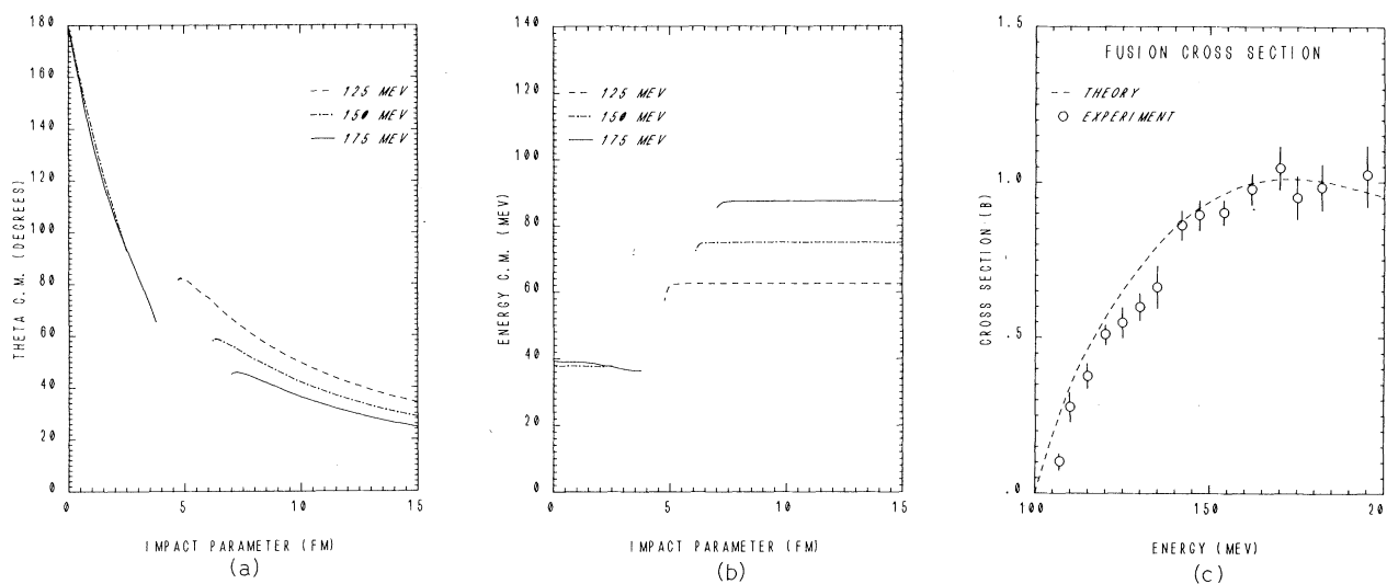
FIG. 2. The reaction ^{40}\text{Ca} + ^{40}\text{Ca} at three different bombarding energies. The theoretical average deflection function, i.e., deflection angle \theta as a function of the impact parameter and the associated energy loss for three cases (125, 150, and 175 MeV) are displayed in (a) and (b), respectively. Both the deflection functions and the energy-loss curves are discontinued for the range of impact parameters where the relative motion displays a second turning point, i.e., a turning point in the outward motion. In this situation the two nuclei remain within the interaction region for a very long time and the collision leads to fusion. The cross section associated with the corresponding range of impact parameters (fusion cross section) is plotted in (c) as a function of the bombarding energy in the laboratory system in comparison with experimental data (Ref. 5).
